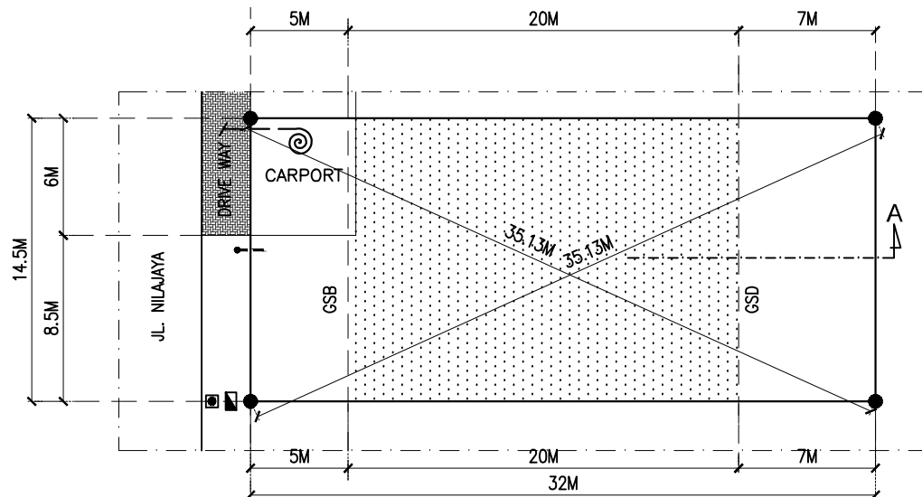
DENAH KAVLING JL. NILAJAYA NO. 27 SKALA 1 : 350
